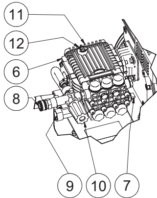
UNLOADER W/BYPASS
